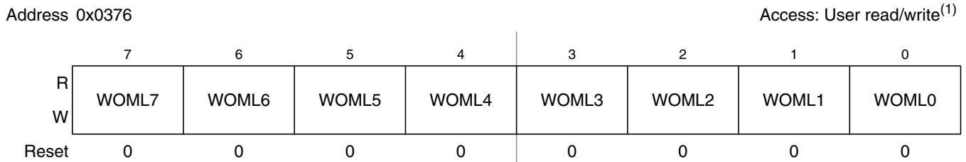
Figure 2-97. Port L Wired-Or Mode Register (WOML)
