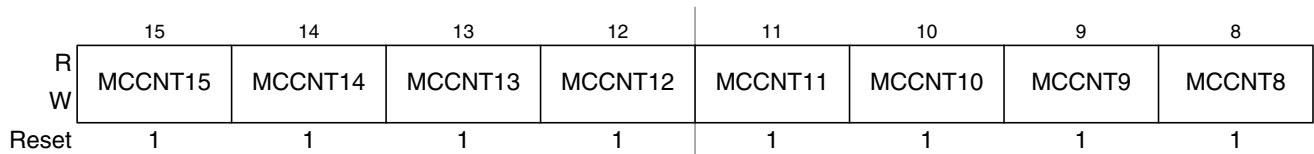
Figure 14-56. Modulus Down-Counter Count Register High (MCCNT)
