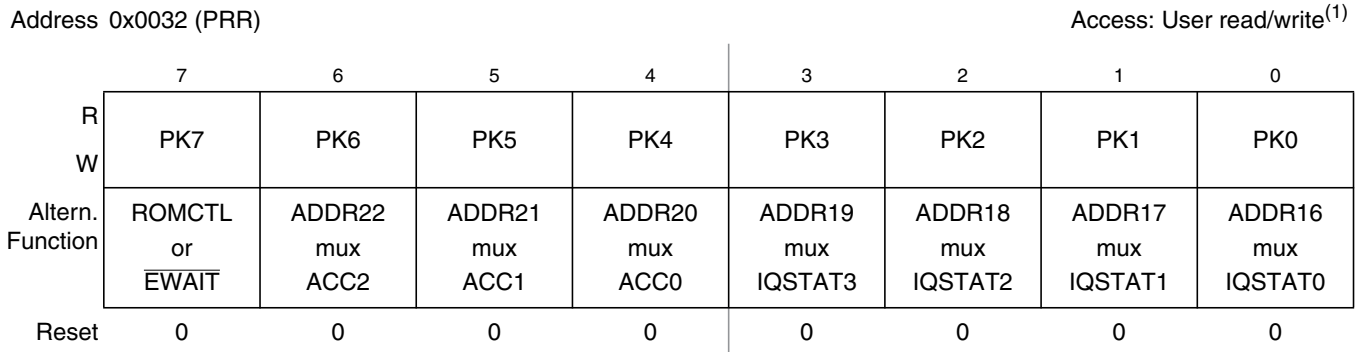
Figure 2-17. Port K Data Register (PORTK)
