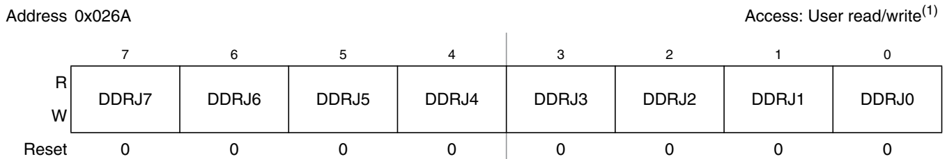
Figure 2-61. Port J Data Direction Register (DDRJ)
