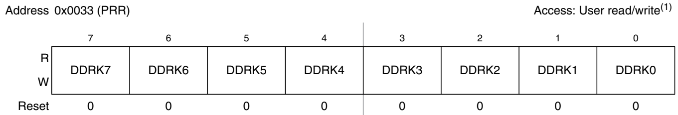
Figure 2-18. Port K Data Direction Register (DDRK)
