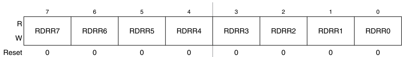
Figure 2-86. Port R Reduced Drive Register (RDRR)
